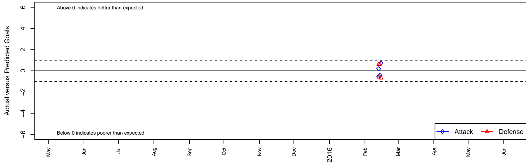
FC United Select 2 B98 Dots are actual minus expected GF (blue circles) and GA (red triangles). Blue line is smoothed change in attack strength. Red is smoothed change in defense strength.
